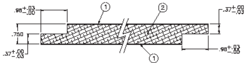
TYPICAL CROSS-SECTION (SHIP-LAP JOINT)
